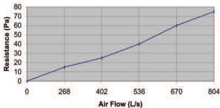
Clean Filter Resistance Vs Air Flow
